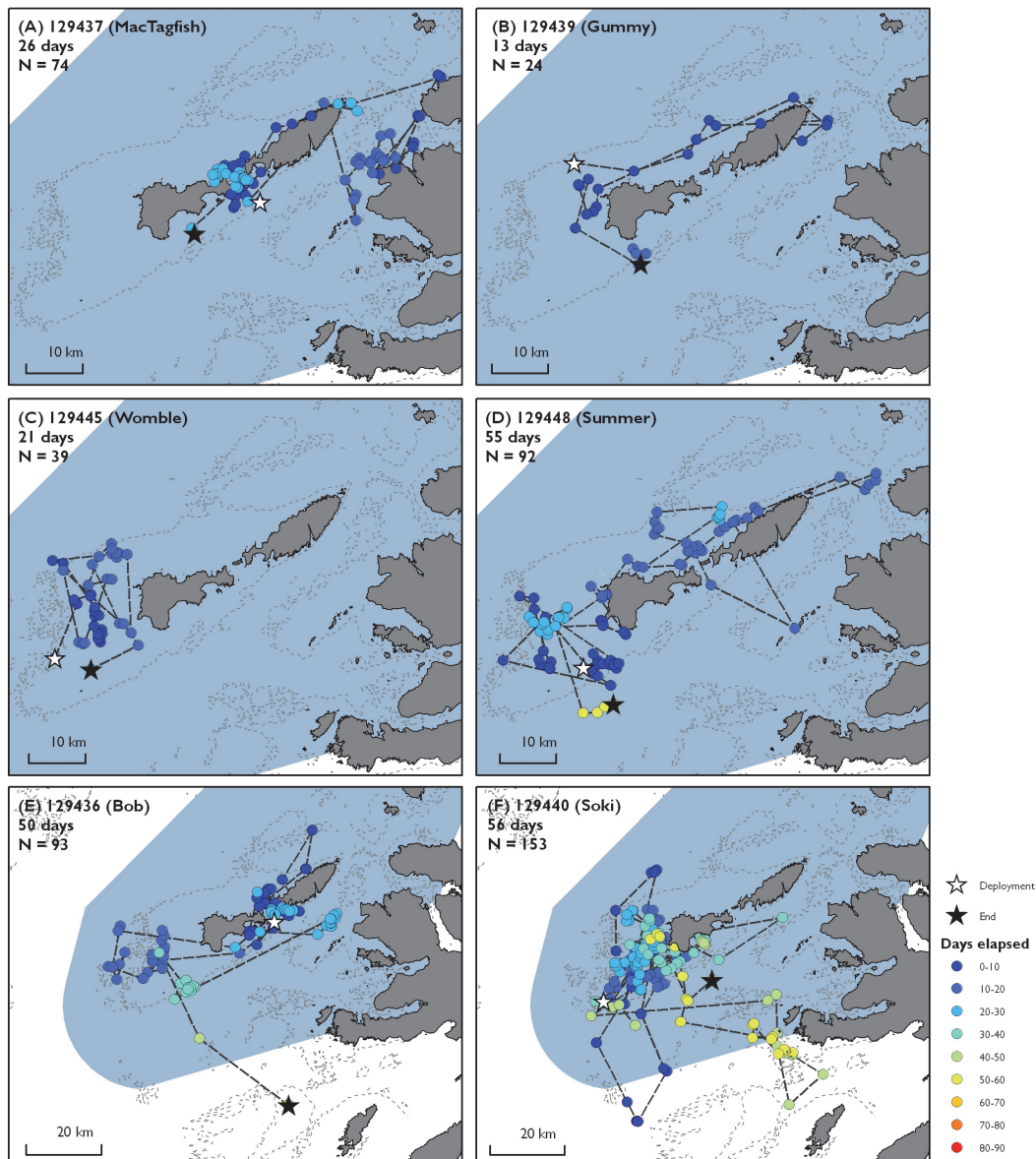
Figure 7. Summertime movements of basking sharks tracked with SPOT tags in 2013. Satellite tracking data from basking sharks satellite tracked between July and September. Shark tag ID, name (if applicable), tracking duration and total number of filtered locations indicated for each figure part. Note figure parts to differing scales. Dashed lines join consecutive locations but do not infer straight line movement. Skye to Mull MPA search location (blue polygon), 50m depth contour (grey broken line; © SeaZone Solutions, 2013, Licence O1035263). Contains Ordnance Survey data © Crown copyright and database right 2013.
