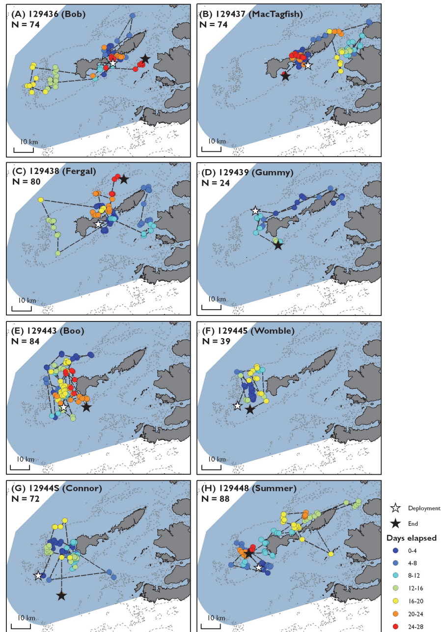
Figure 5. Movements of basking sharks tracked with SPOT tags in 2013. Satellite tracking data from basking sharks for the first 28 days of tracking. Shark tag ID, name and total number of filtered locations indicated for each figure part. Note figure parts to differing scales. Dashed lines join consecutive locations but do not infer straight line movement. Skye to Mull MPA search location (blue polygon), 50m depth contour (grey broken line; © SeaZone Solutions, 2013, Licence O1035263). Contains Ordnance Survey data © Crown copyright and database right 2013.
