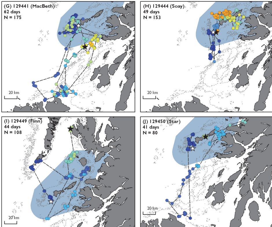
Figure 7 Continued. Summertime movements of basking sharks tracked with SPOT tags in 2013.
