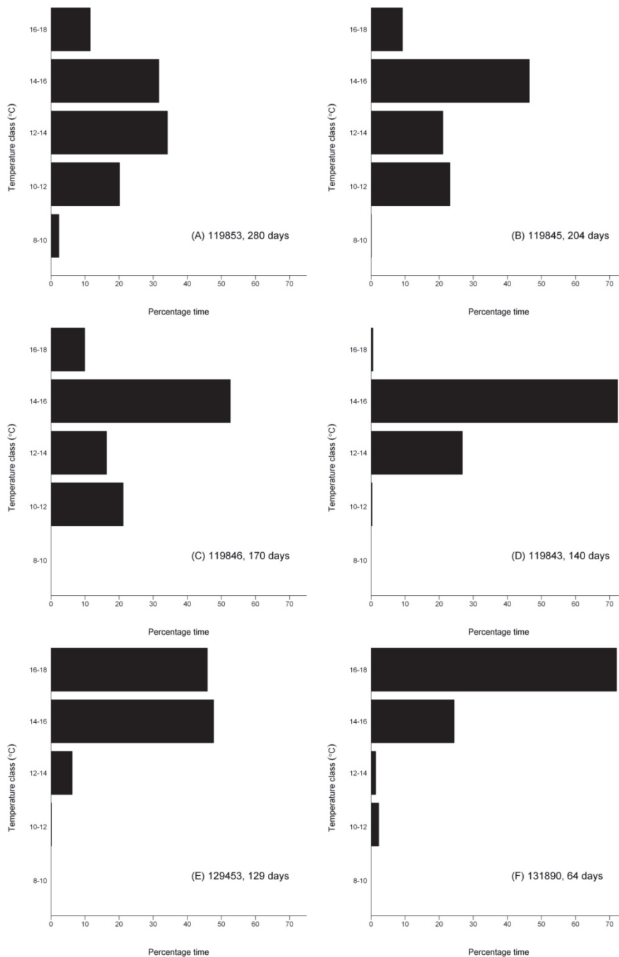
Figure 26. Histograms of time spent in temperature classes. Water temperature encountered by basking sharks tracked by PAT-F (2012; A-D) and MiniPAT tags (2013; E-F); the six tags with the longest attachment durations. Number of days data are indicated with tag ID.
