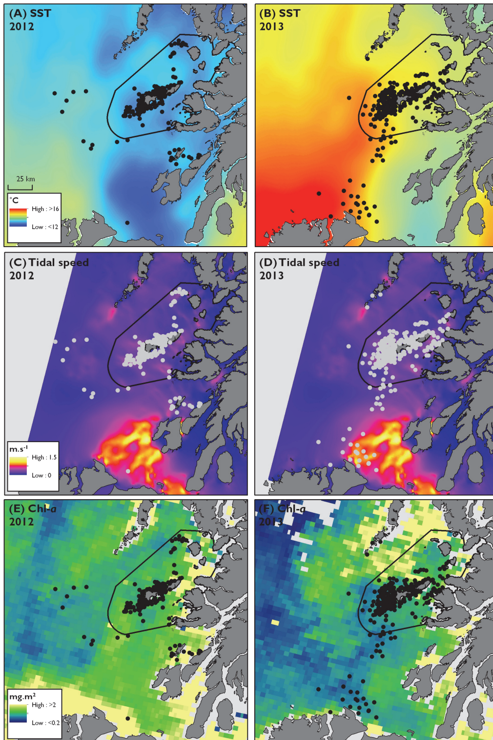
Figure 12. Basking sharks and their environment. First 28 days of satellite tracking locations from individual basking sharks (A, B, E, F black circles and C, D grey circles) in 2012 (A, C and E, N = 8 sharks; N = 177 locations) and in 2013 (B, D and F, N = 15 sharks; N = 313 locations) with respect to sea surface temperature (SST; °C) and tidal speed (m.s -1 ). Mean average of daily data from 13 th July to 11 th August 2012 (A,C), mean average of daily data from 19 th July to 3 rd September 2013 (B,D). Chlorophyll-a concentration (mg.m -2 , mean average of daily data for July 2012 (E) and August 2013 (F). Waters around the tagging areas were considerably warmer in 2013 than in 2012 (A,B) (mean temperature, 13.0°C in 2012 and 14.7°C in 2013). Contains Ordnance Survey data © Crown copyright and database right 2013.
