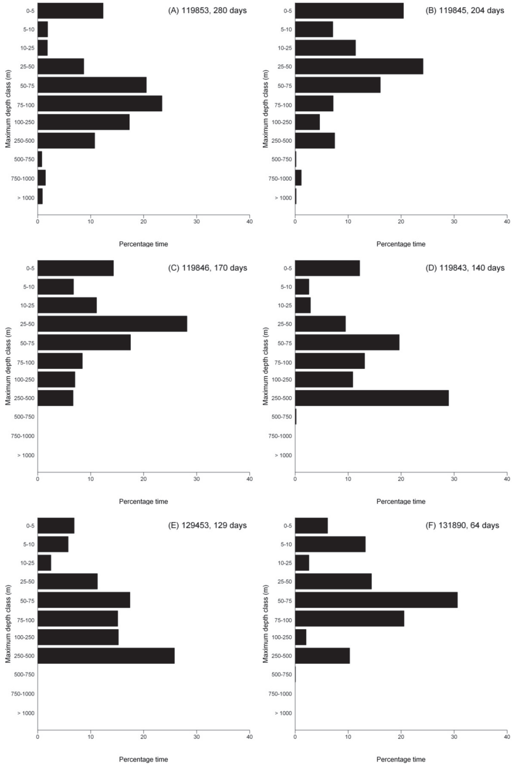
Figure 23. Histograms of time spent in depth classes. Basking shark depth use from PAT-F (2012; A-D) and MiniPAT tags (2013; E-F). The six tags with the longest attachment durations are shown. Number of days data are indicated with tag ID.
