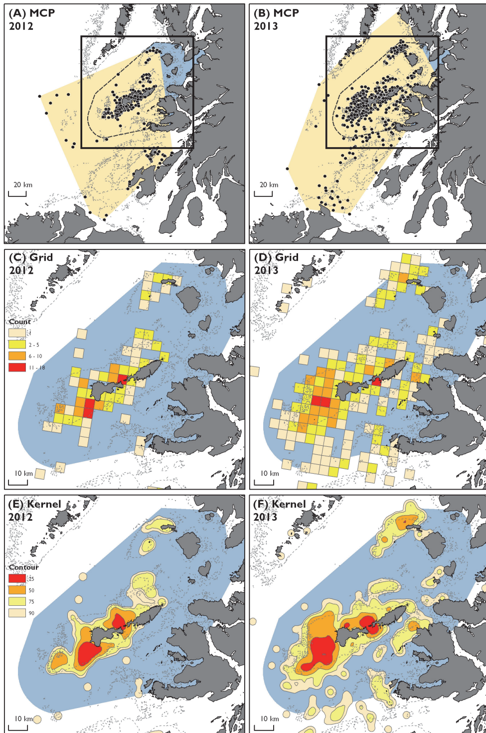
Figure 9. Identifying areas of high relative importance (July to September). Areas of relative importance, estimated using: i) Minimum Convex Polygon (MCP; A,B), ii) Grid; Point density enumeration (C,D) and iii) Kernel; Quartic density estimation (E,F) for SPOT-tagged basking sharks in 2012 (A, C and E) and 2013 (B, D and F) using daily highest quality location from individual basking sharks. Spatial extents of figure parts C-F (black empty polygon) shown in figure parts A and B. Skye to Mull MPA search location (blue polygon), 50m depth contour (grey broken line); © SeaZone Solutions, 2013, Licence O1035263). Contains Ordnance Survey data © Crown copyright and database right 2013.
