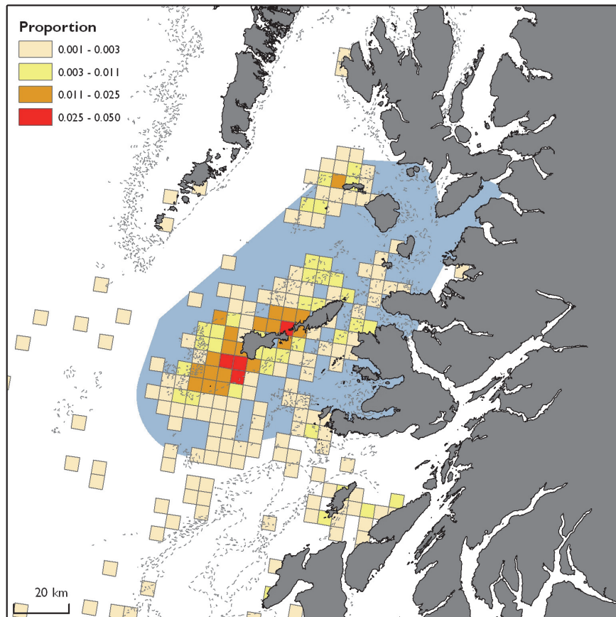
Figure 10. Identifying areas of high relative importance across years. Mean average count as proportions in grid cells across 2012 and 2013 (July to September). Skye to Mull MPA search location (blue polygon), 50m depth contour (grey broken line); (grey broken line; © SeaZone Solutions, 2013, Licence O1035263). Contains Ordnance Survey data © Crown copyright and database right 2013.
