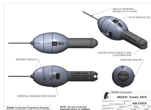
Figure 2. Animal-borne satellite tag technologies (Images: Wildlife Computers).
