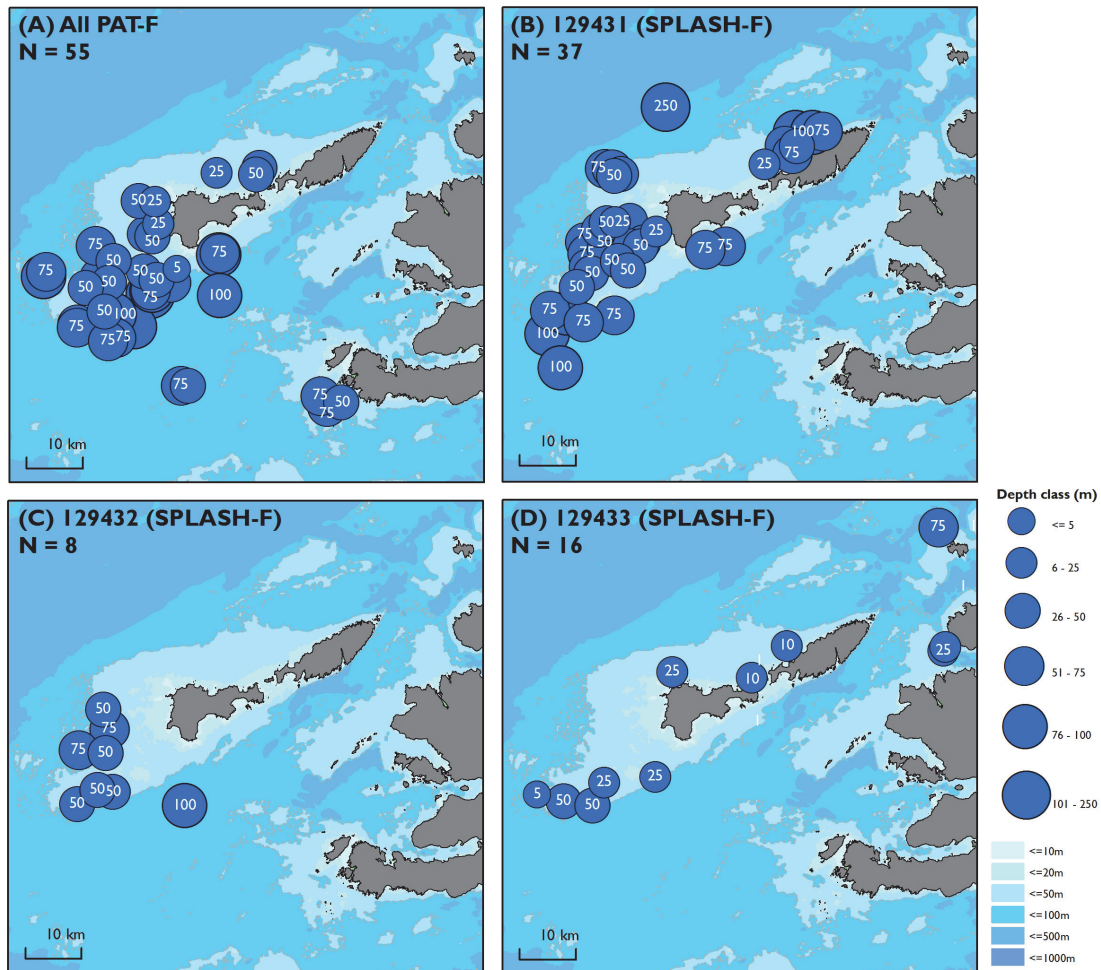
Figure 18. Three dimensional space use from PAT-F (2012; N = 6) and SPLASH-F tags (2013; N = 3). Maximum depth recorded during dives where a temporally coincident Fastloc™ location was available. Circle size indicates dive depth (deeper dives represented by larger circles). Maximum depth value indicated in circle in white text. Background shading shows bathymetry (© SeaZone Solutions, 2013, Licence O1035263). Contains Ordnance Survey data © Crown copyright and database right 2013.
