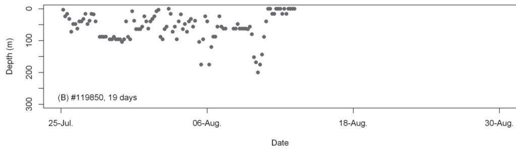
Figure S3. Maximum depths recorded at 4-hour intervals. Maximum depths (filled circles) from 4-hour summary intervals [non-contiguous] collected by PAT-F tags.
