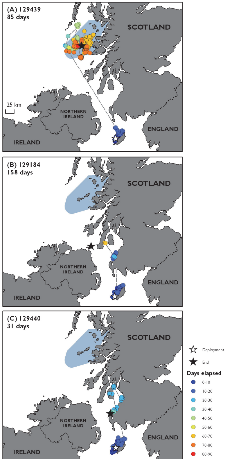
Figure 27. Movements of basking sharks tracked with SPOT tags in 2012 from the Isle of Man. Satellite-derived locations from basking sharks tagged in the water surrounding the Isle of Man. Shark tag ID, name (if applicable) and attachment duration indicated for each figure part. Note one basking shark (A) transmits from within the Skye to Mull search location. Dashed lines join consecutive locations but do not infer straight line movement. Skye to Mull MPA search location (blue polygon). Contains Ordnance Survey data © Crown copyright and database right 2013.
