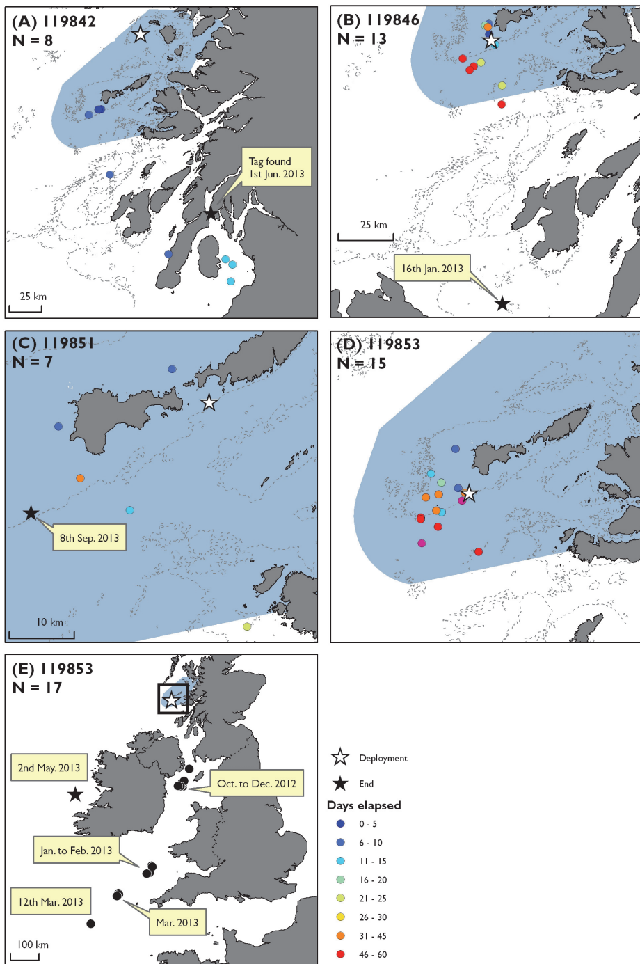
Figure 14. Fastloc™ locations of four PAT-F tagged basking sharks in 2012. PAT-F tag attachment locations (white stars), PAT-F tag pop-off locations (black stars). Insufficient locations were transmitted to estimate density, see also Fig. S2 for locations from tags collecting four or less Fastloc™ locations. Locations from tag 119853 are displayed across two figure parts (D: locations in the area of the Skye to Mull search locations and E: locations from southward migration through the Irish and Celtic Seas (with positions in E shown as black circles). Number of successfully derived locations given with tag ID. Skye to Mull MPA search location (blue polygon). 50m depth contour (grey broken line; © SeaZone Solutions, 2013, Licence O1035263). Contains Ordnance Survey data © Crown copyright and database right 2013.
