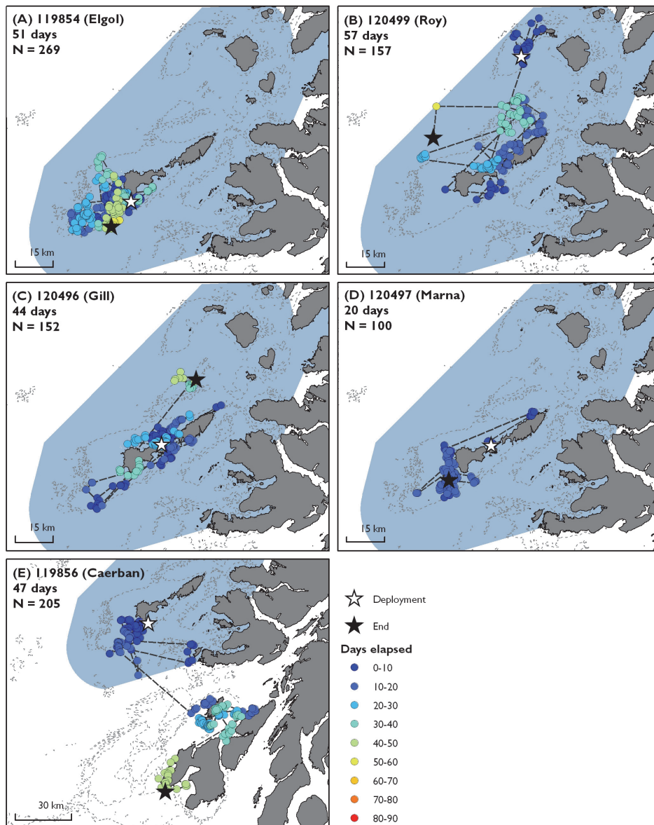
Figure 6. Summertime movements of basking sharks tracked with SPOT tags in 2012. Satellite tracking data from basking sharks satellite tracked between July and September. Shark tag ID, name (if applicable), tracking duration and total number of filtered locations indicated for each figure part. Note figure parts to differing scales. Dashed lines join consecutive locations but do not infer straight line movement. Skye to Mull MPA search location (blue polygon), 50m depth contour (grey broken line; © SeaZone Solutions, 2013, Licence O1035263). Contains Ordnance Survey data © Crown copyright and database right 2013.
