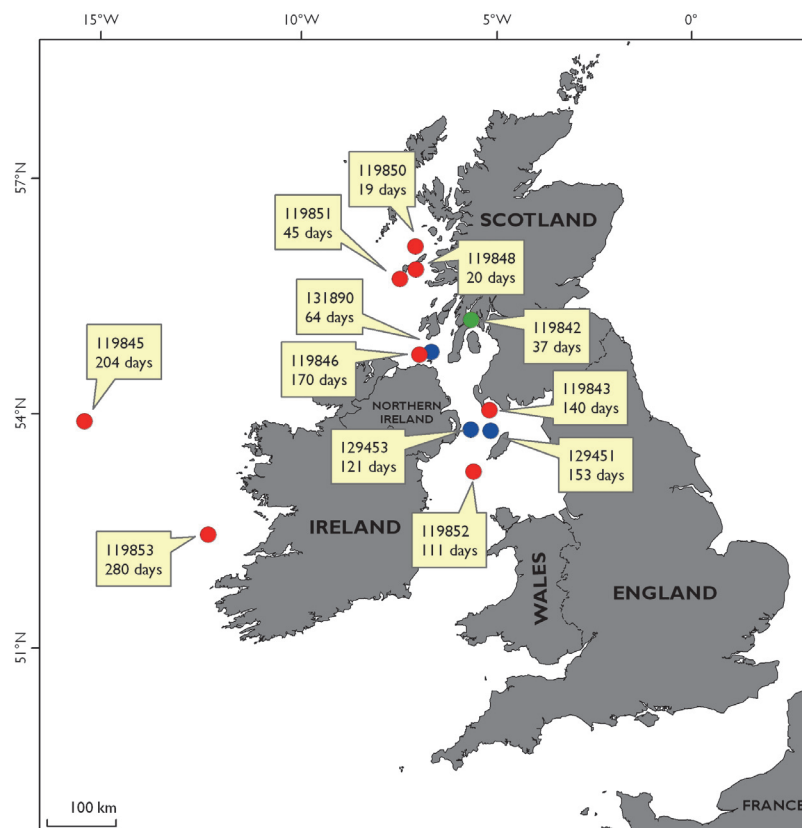
Figure 16. PAT-F and MiniPAT satellite tag detachment locations. Pop-off locations of PAT-F tags (red circles; N = 8 ), MiniPAT tags (blue circles; N = 3 ) and retrieval location of a non-transmitting PAT-F tag (green circle, N = 1 ). Attachment durations given with tag ID.
