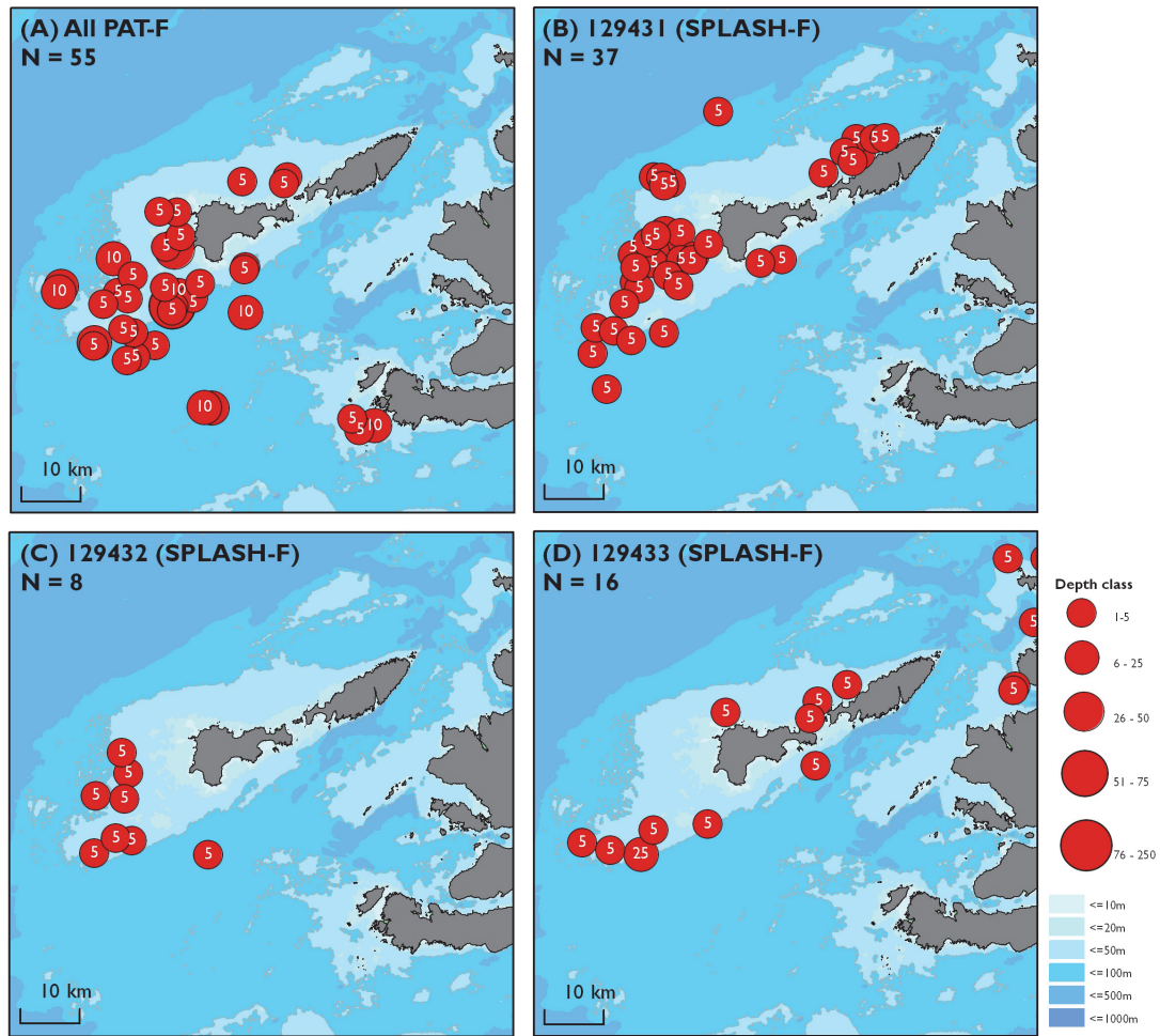
Figure 19. Three dimensional space use from PAT-F (2012; N = 6) and SPLASH-F tags (2013; N = 3). Most frequent depth class occupied during dives where a temporally coincident Fastloc™ location was available. Circle size indicates depth class (deeper dives represented by larger circles). Most frequent depth class indicated in circle in white text. Background shading shows bathymetry (© SeaZone Solutions, 2013, Licence O1035263). Contains Ordnance Survey data © Crown copyright and database right 2013.
