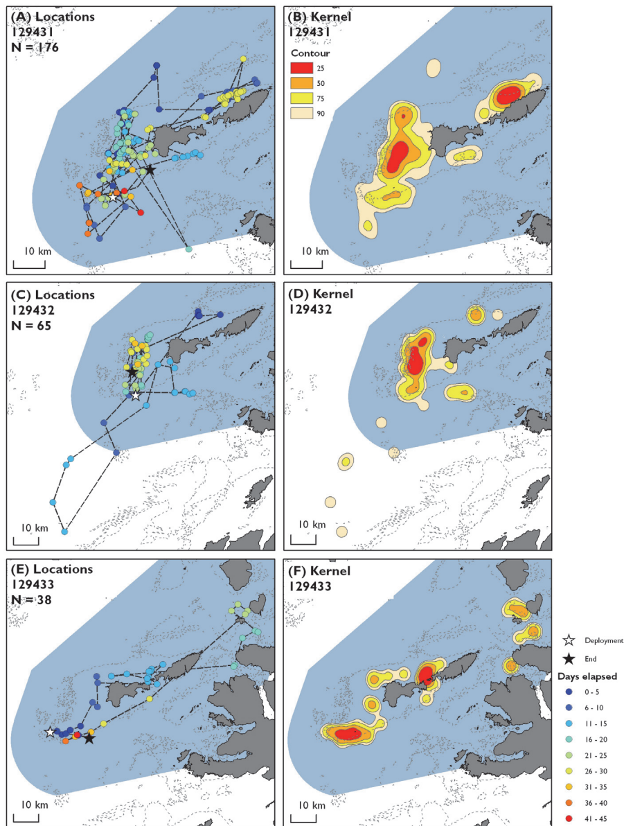
Figure 15. Fastloc™ locations of three SPLASH-F tagged basking sharks in 2013. GPS locations (A, C and E), and resulting density (B, D and F) estimated using quartic density estimation. Attachment location (white star), SPLASH-F tag pop-off locations derived from first received Argos location following detachment (black star). Shark tag ID, name (if applicable), tracking duration and total number of filtered locations indicated for each figure part. Note figure parts to differing scales. Dashed lines join consecutive locations but do not infer straight line movement. Skye to Mull MPA search location shown (blue polygon), 50m depth contour (grey broken line; © SeaZone Solutions, 2013, Licence O1035263). Contains Ordnance Survey data © Crown copyright and database right 2013.
