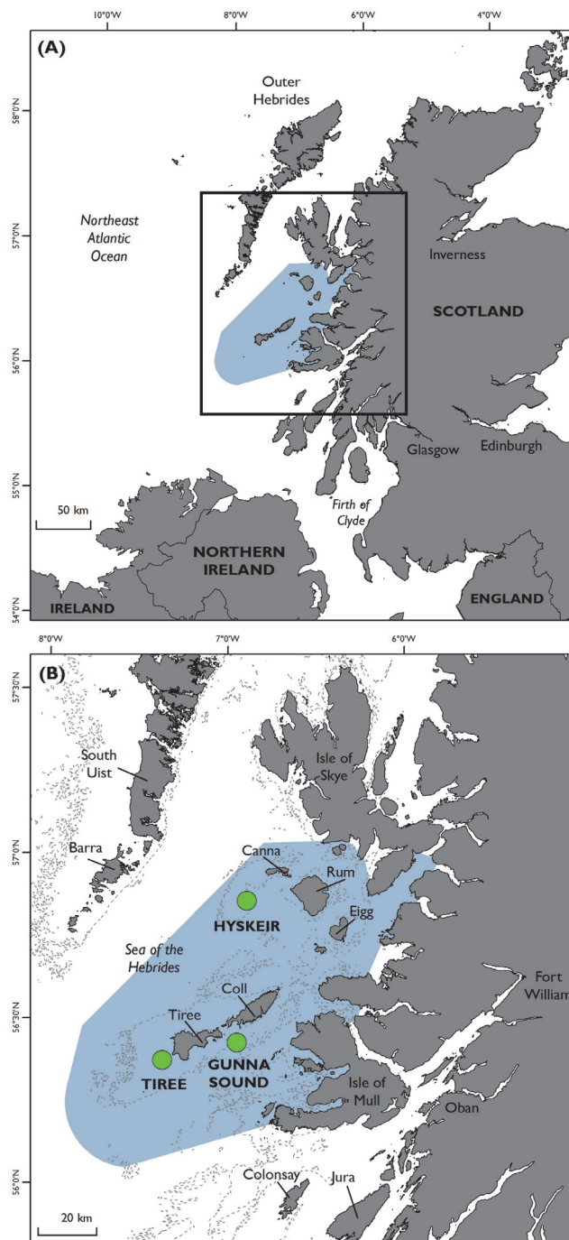
Figure 1. (A) Study location; west coast of Scotland, showing Skye to Mull MPA search location (blue polygon) in the Sea of the Hebrides and (B) Satellite tag deployment areas in 2012 and 2013 (Hyskeir, Gunna Sound and Tiree; green circles). 50m depth contour (grey broken line; © SeaZone Solutions, 2013, Licence O1035263). Contains Ordnance Survey data © Crown copyright and database right 2013.
