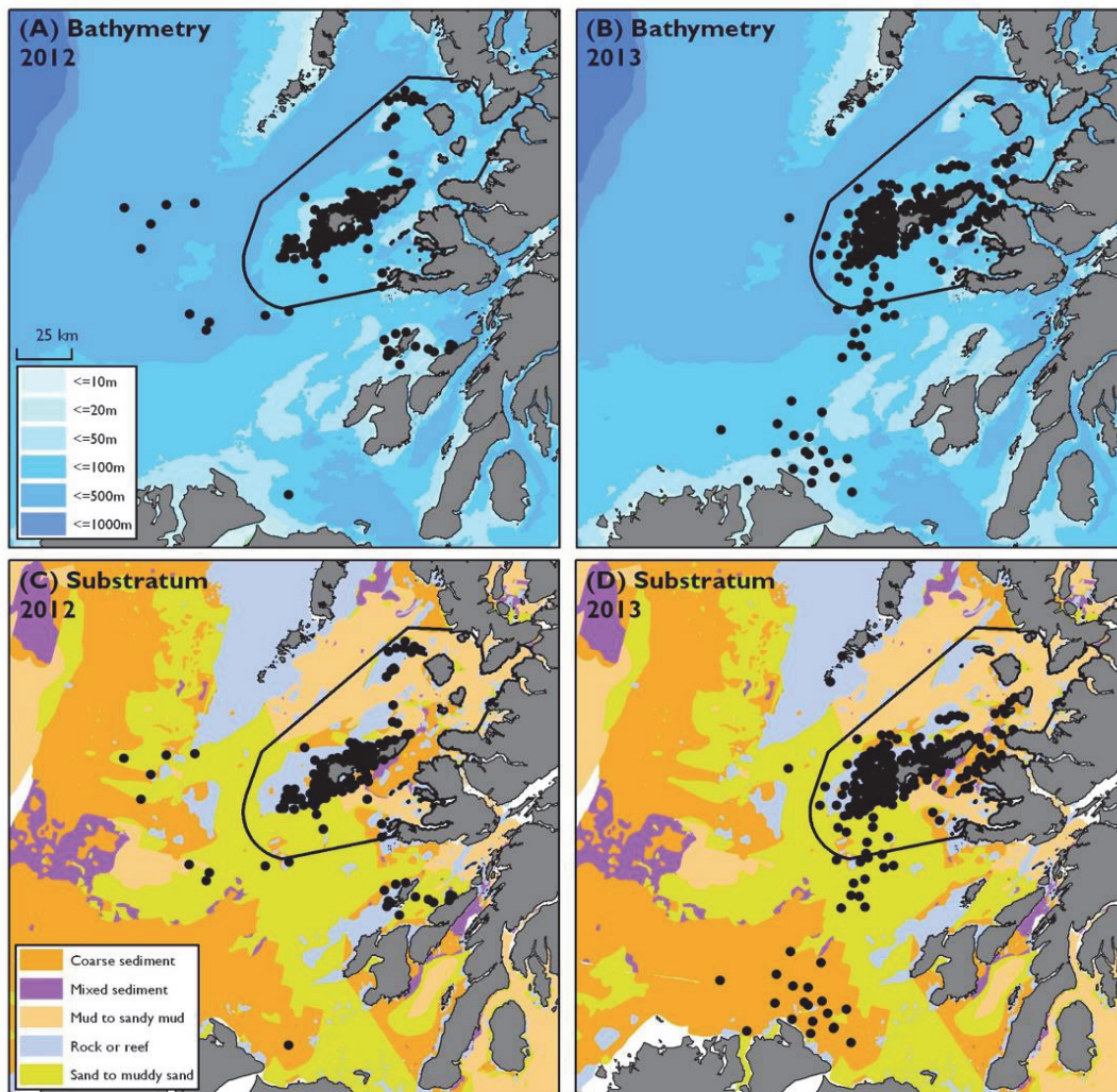
Figure 11. Basking sharks and their environment. First 28 days of satellite tracking locations from individual basking sharks (black circles) in 2012 (A and C; N = 8 sharks; N = 177 locations) and 2013 (B and D; N = 15 sharks; N = 313 locations) with respect to bathymetry (m; A,B) and seabed substratum (C,D). In the first 28 days of tracking sharks are predominantly located in waters less than 50m deep (A,B) and over rock or reef substratum (C,D). Contains Ordnance Survey data © Crown copyright and database right 2013. Bathymetry © SeaZone Solutions, 2013, Licence O1035263.
