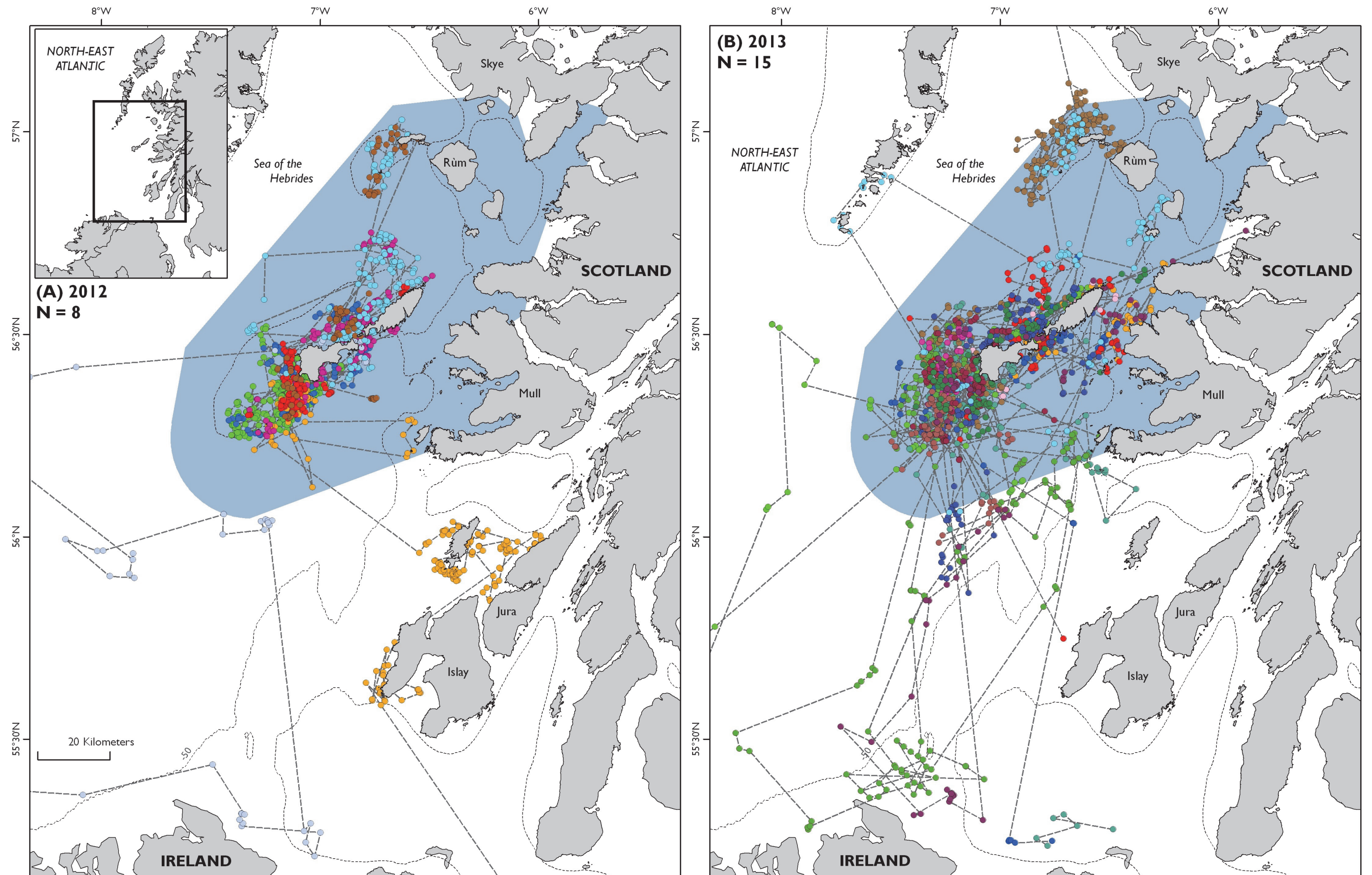
Figure S1. Satellite tracking locations of basking sharks gathered in the Sea of the Hebrides from SPOT tags during (A) 2012 and (B) 2013. Individual shark locations represented by single colour points, dashed line joins consecutive locations. Skye to Mull MPA search location (blue polygon). Contains Ordnance Survey data © Crown copyright and database right 2013.
