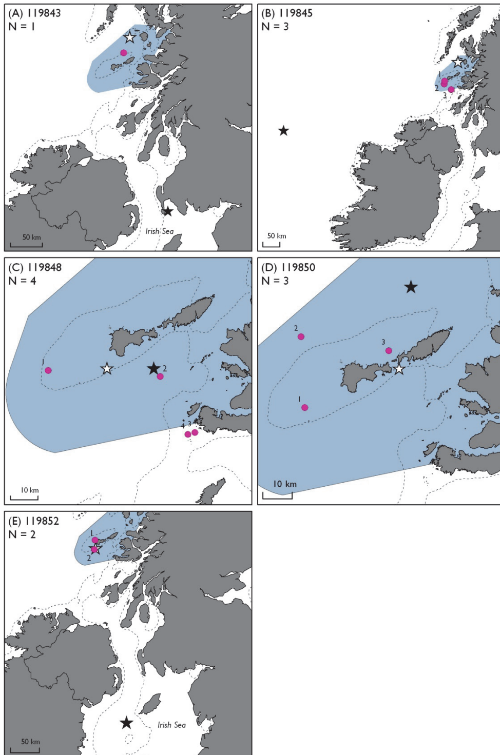
Figure S2. GPS locations of basking sharks from PAT-F tags in 2012. GPS locations gathered from tags producing 4 or less. GPS locations sequentially numbered in order of occurrence. PAT-F tag attachment locations (empty stars), PAT-F tag pop-off locations (filled stars). Number of locations given with tag ID. Skye to Mull MPA search location shown (blue polygon). 50m depth contour (broken grey line; GEBCO). Contains Ordnance Survey data © Crown copyright and database right 2013.
