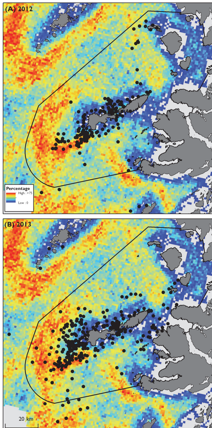
Figure 13. Basking sharks and fronts. Locations of basking sharks in the first 28 days of tracking (black circles) in 2012 (A) and 2013 (B) with respect to persistent fronts. Background image indicates persistence of horizontal surface thermal fronts (data from Defra MB0102 Project (Report No. 20, Miller et al. 2010). Skye to Mull MPA search location (black empty polygon). Contains Ordnance Survey data © Crown copyright and database right 2013.
