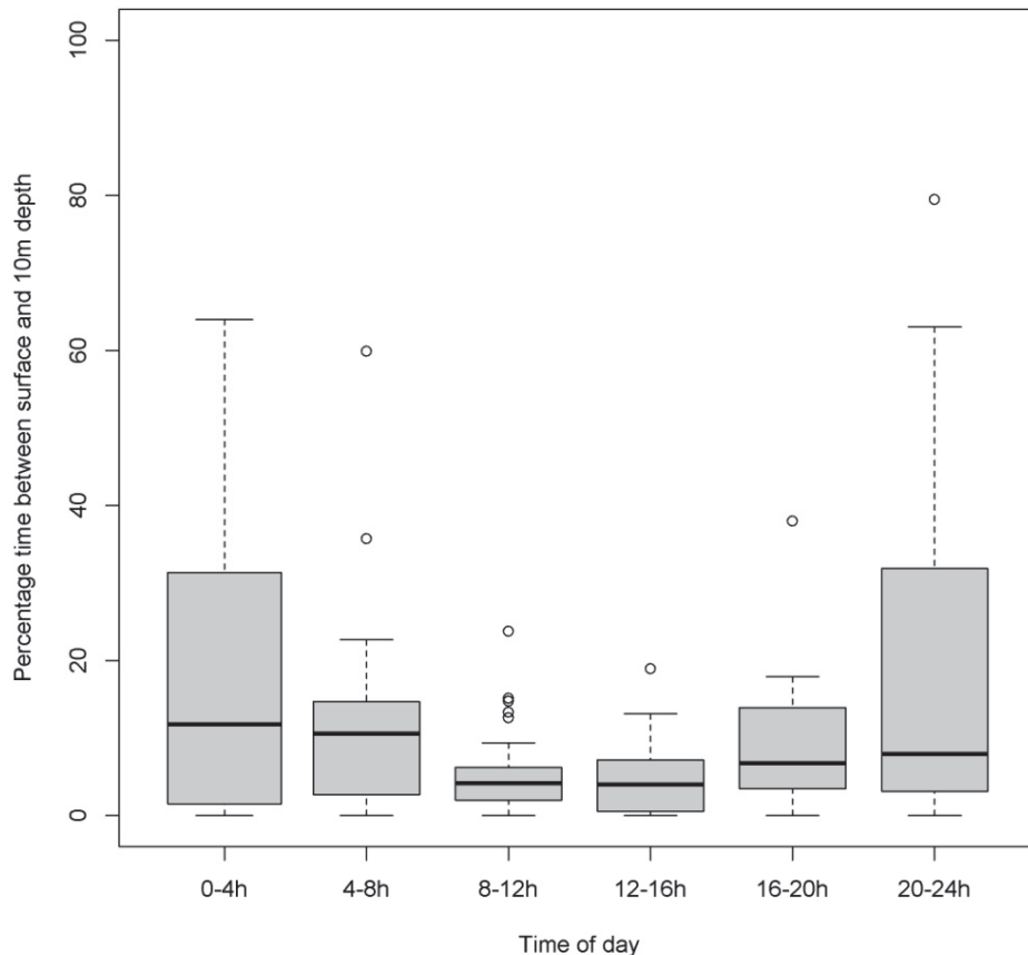
Figure 21. Basking shark depth use with time of day in the Sea of the Hebrides in 2012. Percentage time spent between the surface and 10m depth within the first 28 days of PAT-F tag deployments (N = 9 basking sharks) summarised at 4-hour intervals. Each box represents the range of values observed from received data for the relevant time period. The bold horizontal line represents the median value for each vertical box, upper and lower extent of each box represents the 25 th and 75 th percentiles respectively. Dashed vertical lines extending from the top and bottom of the boxes indicate the range of values in the distribution to approximately the 2.5 th to 97.5 th percentiles. Open circles represent outliers; these are values occurring outside the 2.5 th and 97.5 th percentiles of data distribution.
