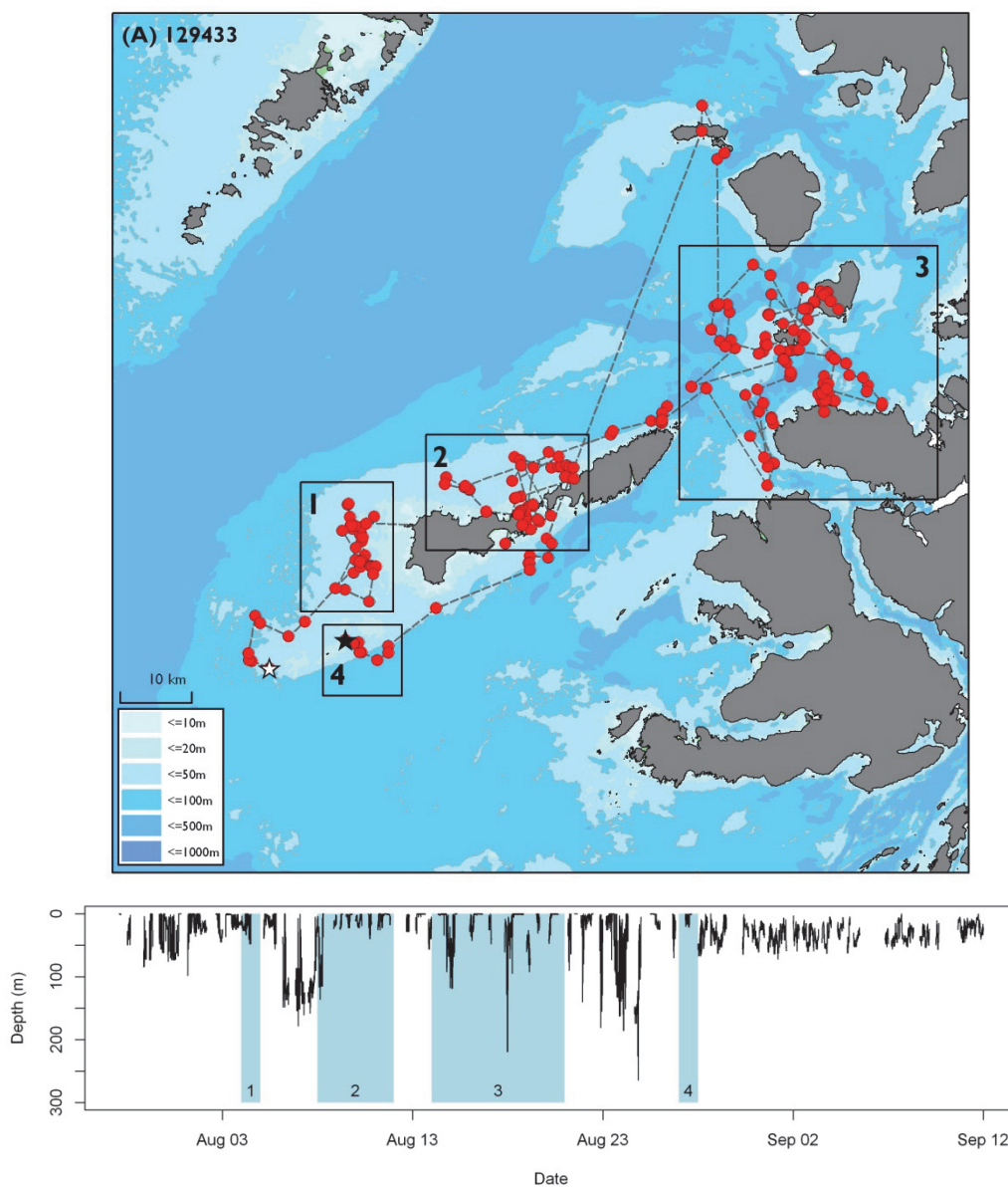
Figure 20. Basking shark depth use from SPLASH-F tags in 2013. Locations of basking sharks tracked with a SPLASH-F tag (red circles; upper panel). First location received following tagging (white star), final location received (black star). Average depths recorded at 5-min. intervals (lower panel). Numbered regions in map correspond to
