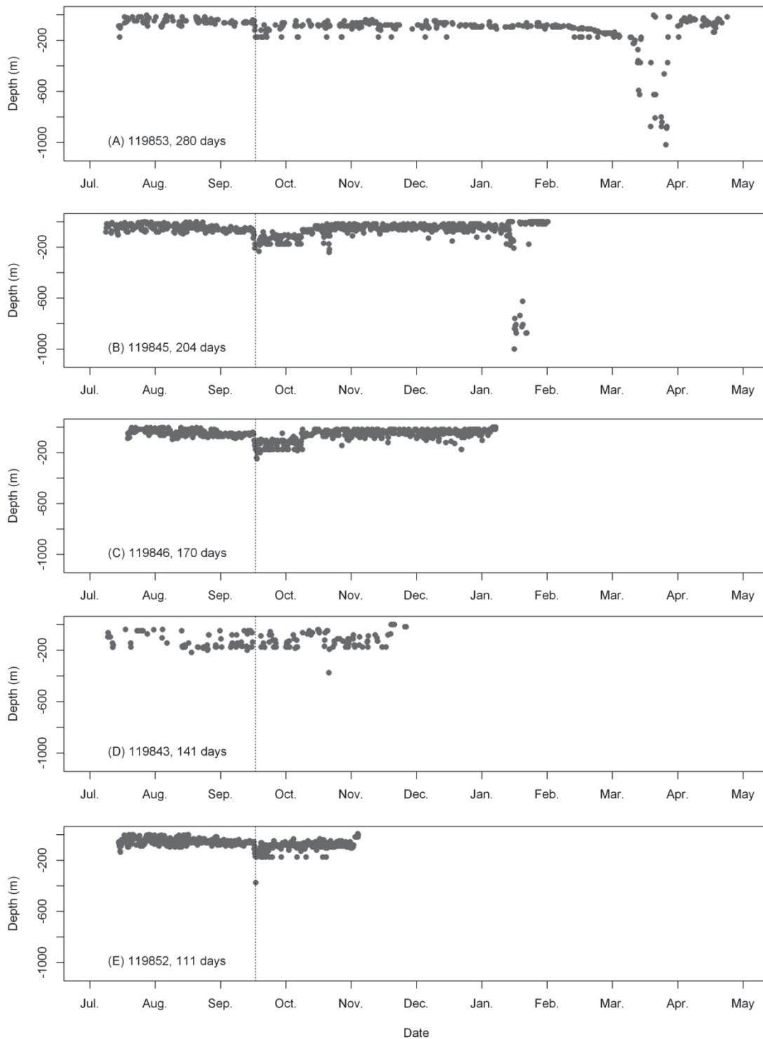
Figure 24. Maximum depths recorded at 4-hour intervals. Maximum depths (filled circles) from 4-hour summary intervals [non-contiguous] from five of the longest depth use time series collected by PAT-F tags in 2012. Tags sorted by decreasing attachment duration. Vertical dashed line indicates the 30th of September 2012 where depth-use behaviour appears to change across individuals. The majority of dives were to less than 200m and deeper dives (more than 500m) tend to occur mid-winter to spring. See also Figure S3 for dive data from PAT-F tags with deployments 20 days or less.
