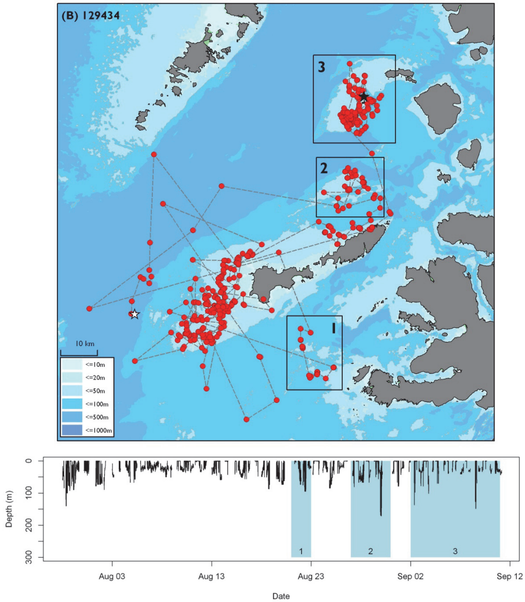
Figure 20 Continued. Basking shark depth use from SPLASH-F tags in 2013.
