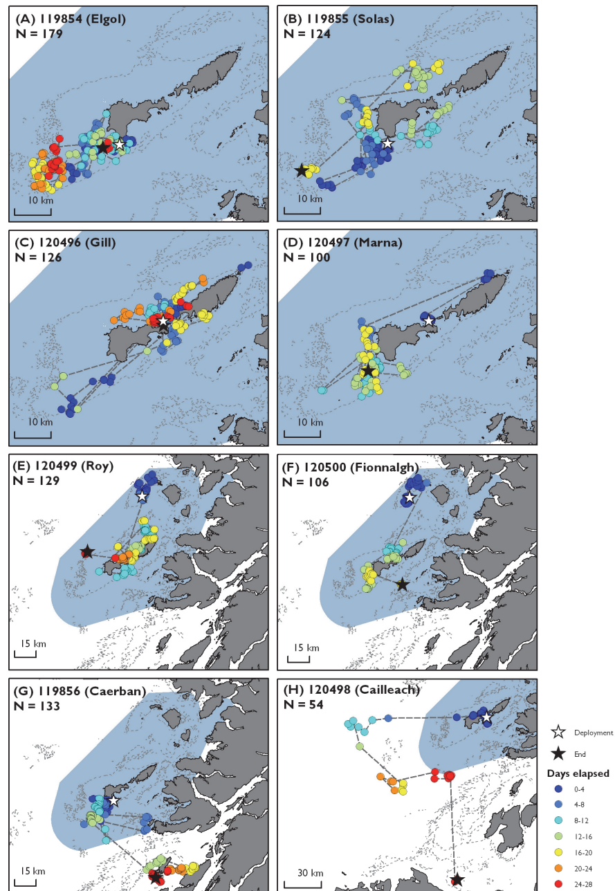
Figure 4. Movements of basking sharks tracked with SPOT tags in 2012. Satellite tracking data from basking sharks for the first 28 days of tracking. Shark tag ID, name and total number of filtered locations indicated for each figure part. Note three basking sharks were tracked for less than 28 days (B, D and F) and figure parts to differing scales. Dashed lines join consecutive locations but do not infer straight line movement. Skye to Mull MPA search location (blue polygon), 50m depth contour (grey broken line; © SeaZone Solutions, 2013, Licence O1035263). Contains Ordnance Survey data © Crown copyright and database right 2013.
