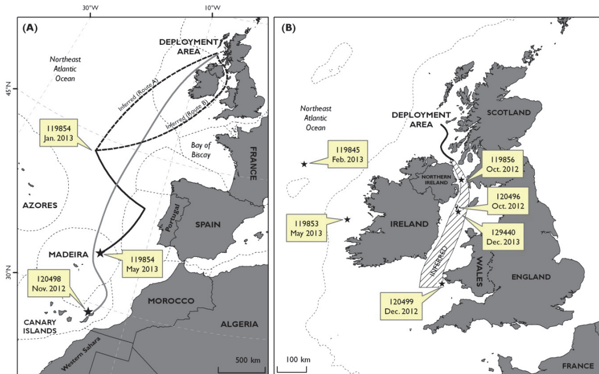
Figure 17. Long and medium-range movements of basking sharks from Scotland. (A) Two SPOT-tagged basking sharks in 2012 (119854, 120498). (B) Boundaries of Exclusive Economic Zones (black dashed line). Three SPOT (119856, 120496 and 120499) and two PAT-F (119845, 119853) tagged basking sharks in 2012 and one SPOT (129440) tagged basking shark in 2013 moving in to the Irish and Celtic seas from the Sea of the Hebrides. Hatched region (B) identifies an inferred movement corridor stretching from Scotland to the Celtic Sea. Month of tag detachment indicated with tag ID. 200m depth contour (grey broken line); (grey broken line; © SeaZone Solutions, 2013, Licence O1035263). Contains Ordnance Survey data © Crown copyright and database right 2013
