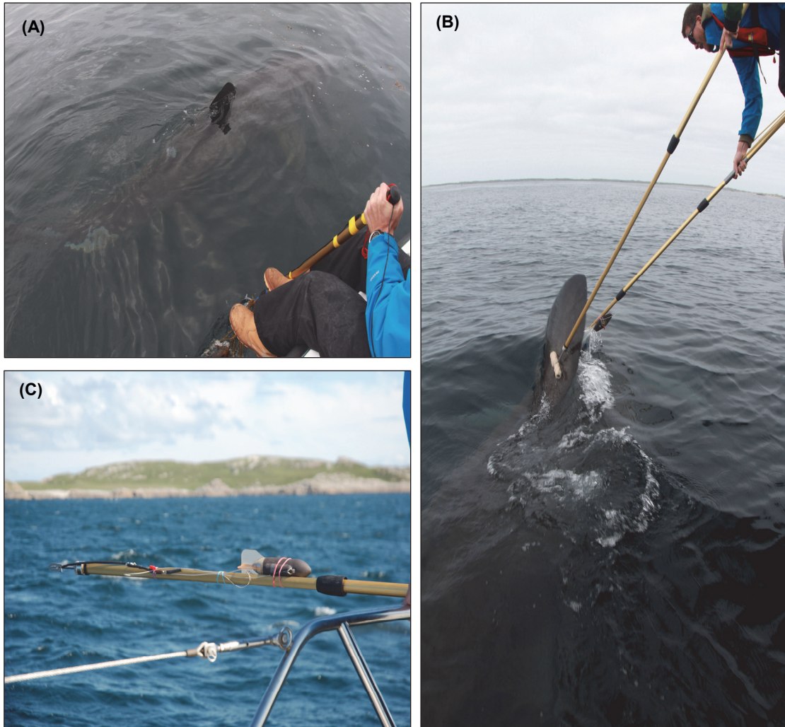
Figure 3. Use of pole mounted camera to determine sex of satellite tagged basking sharks (A), genetic swab pole and darting pole being used simultaneously (B) and darting pole with satellite tag and tether prepared for use (C).
