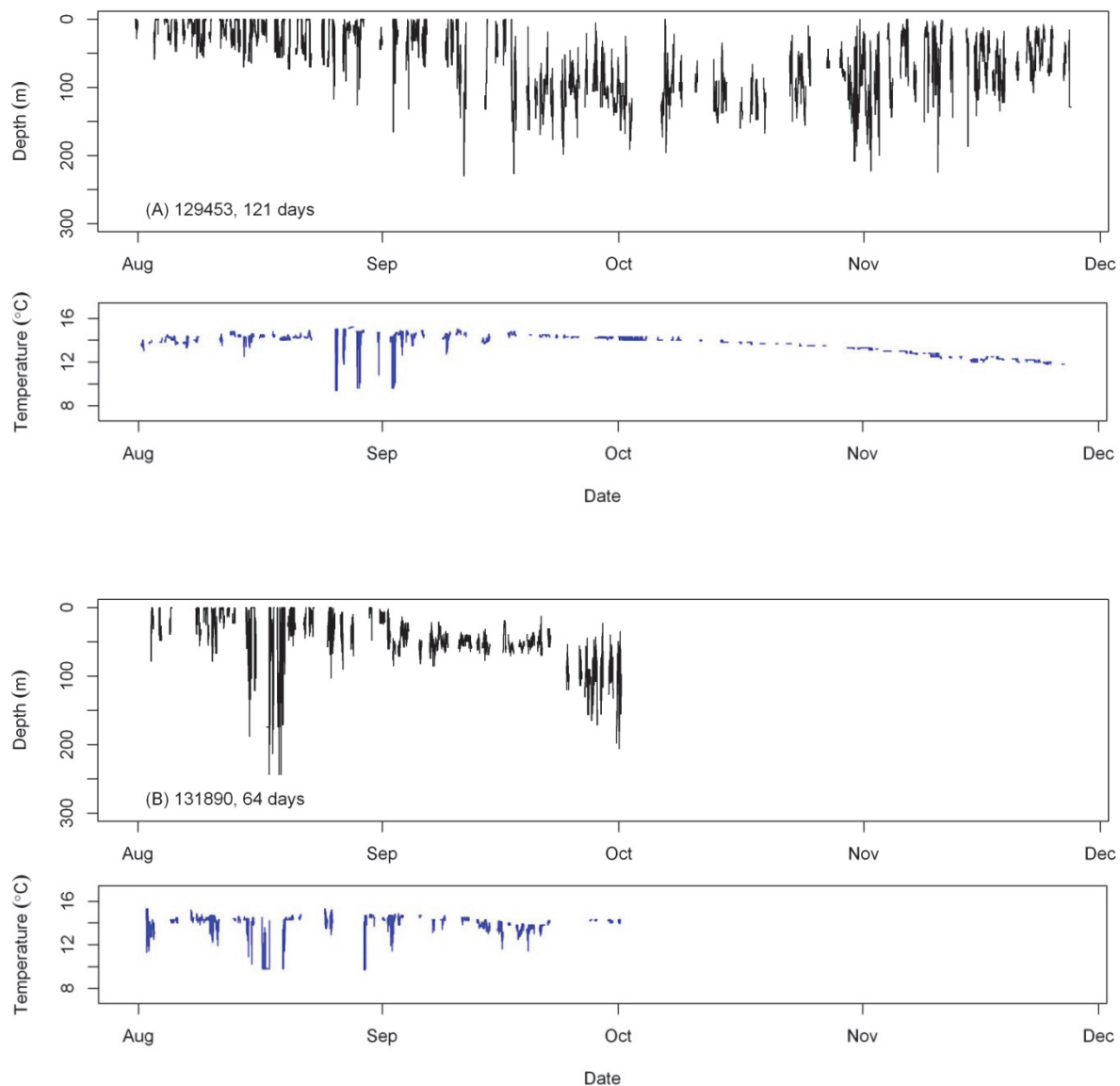
Figure 25. Basking shark depth utilisation and ambient environmental temperature time-series from MiniPAT in 2013. Mean depths (upper panels; black line) and mean temperatures (lower panels; blue line) calculated at ten-minute intervals [non-contiguous] from two prematurely detached MiniPAT tags. Tags sorted by decreasing attachment duration.
