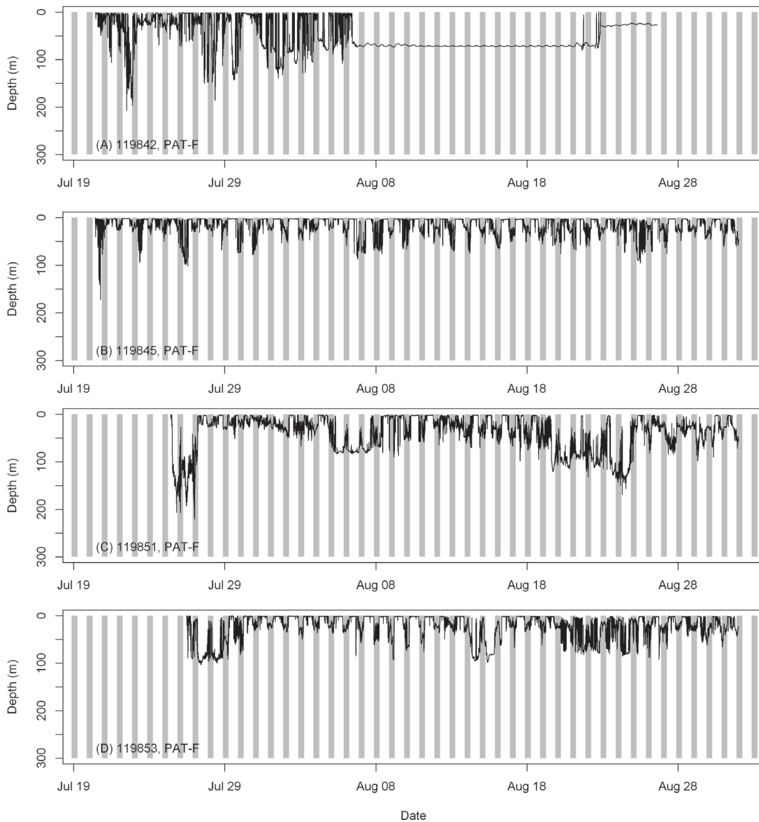
Figure 22. Basking shark depth use time series from physically recovered PAT-F, SPLASH-F and MiniPAT tags. Depth recorded at a 10-second frequency and summarised at 5 min. intervals from physically recovered tags. All figures plots displayed for period between 19 th July and 28 th August (N = 40 days). Grey bars indicate period between mean civil sunset and mean sunrise (9-hours duration, starting at 9pm daily) for the period.
