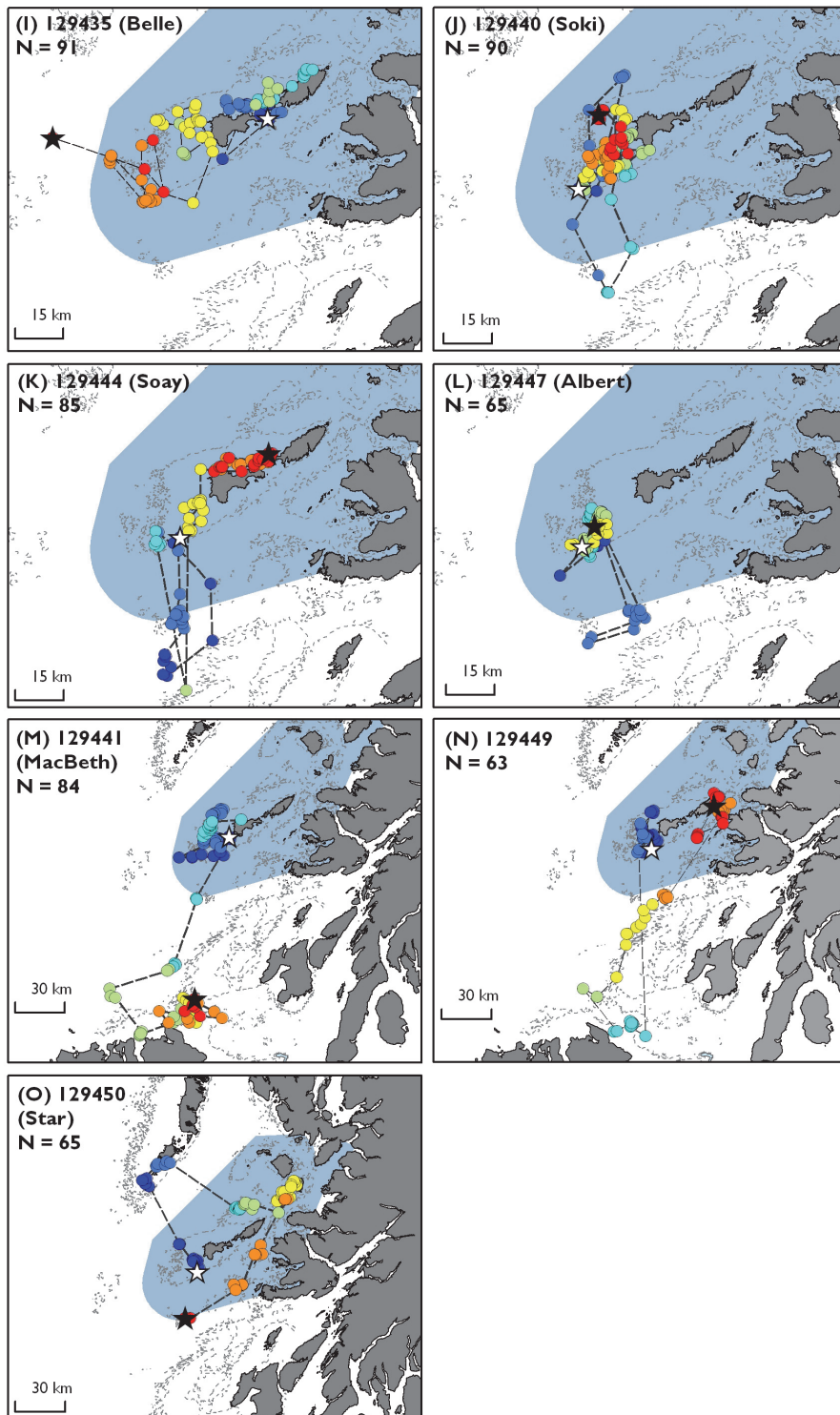
Figure 5 Continued. Movements of basking sharks tracked with SPOT tags in 2013.
