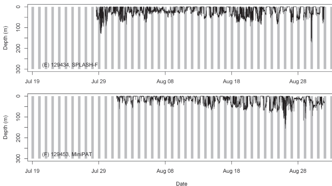
Figure 22. Continued. Basking shark depth use time series from physically recovered PAT-F, SPLASH-F and MiniPAT tags.
