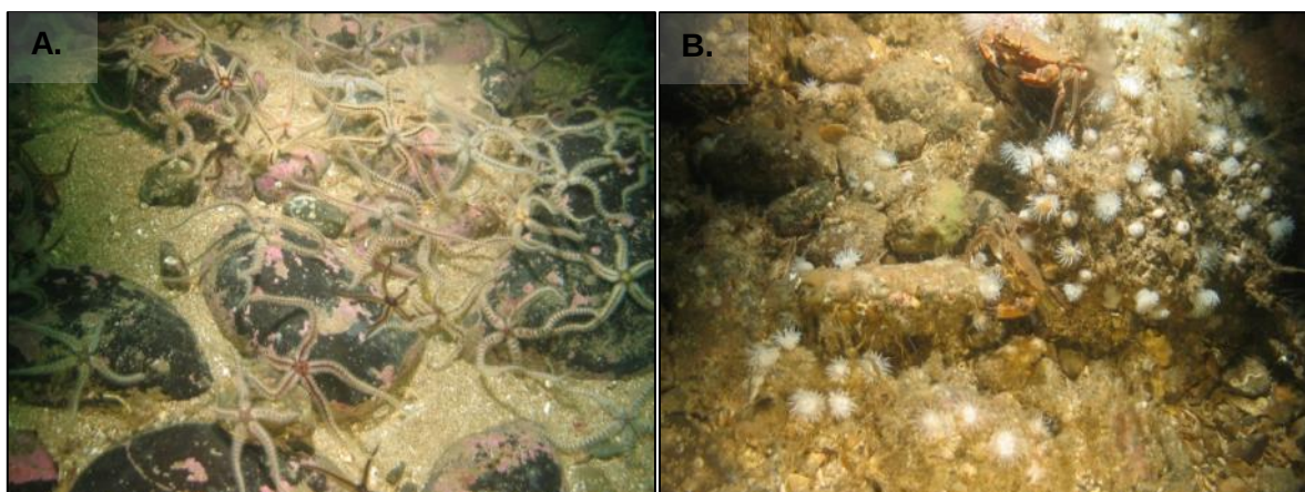
Figure 11. Example images of circalittoral rock biotopes from the mouth of Luce Bay. A. CR.MCR.EcCr.FaAlCr.Bri , LB413; B. CR.HCR.XFa.ByErSp.DysAct , LB420.
