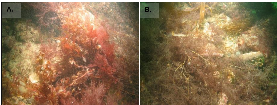
Figure 9. Example images of IR.HIR.KSed biotopes from the south-western coastline. A. LB305; B. LB318.
