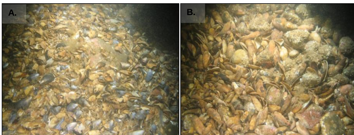
Figure 32. Example images of dead mussel shell aggregations. A. LB518; B. LB513.
