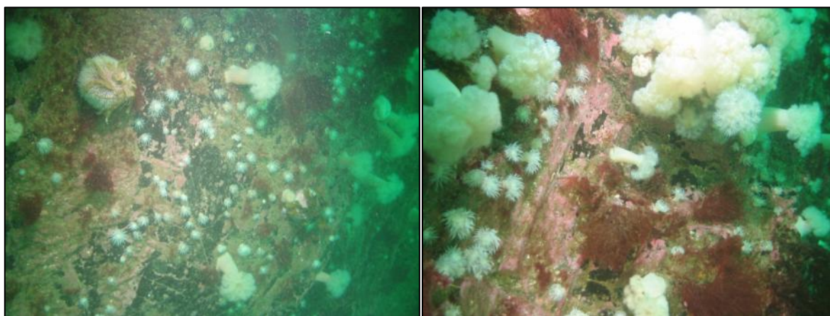
Figure 19. Example images of station LB407.
