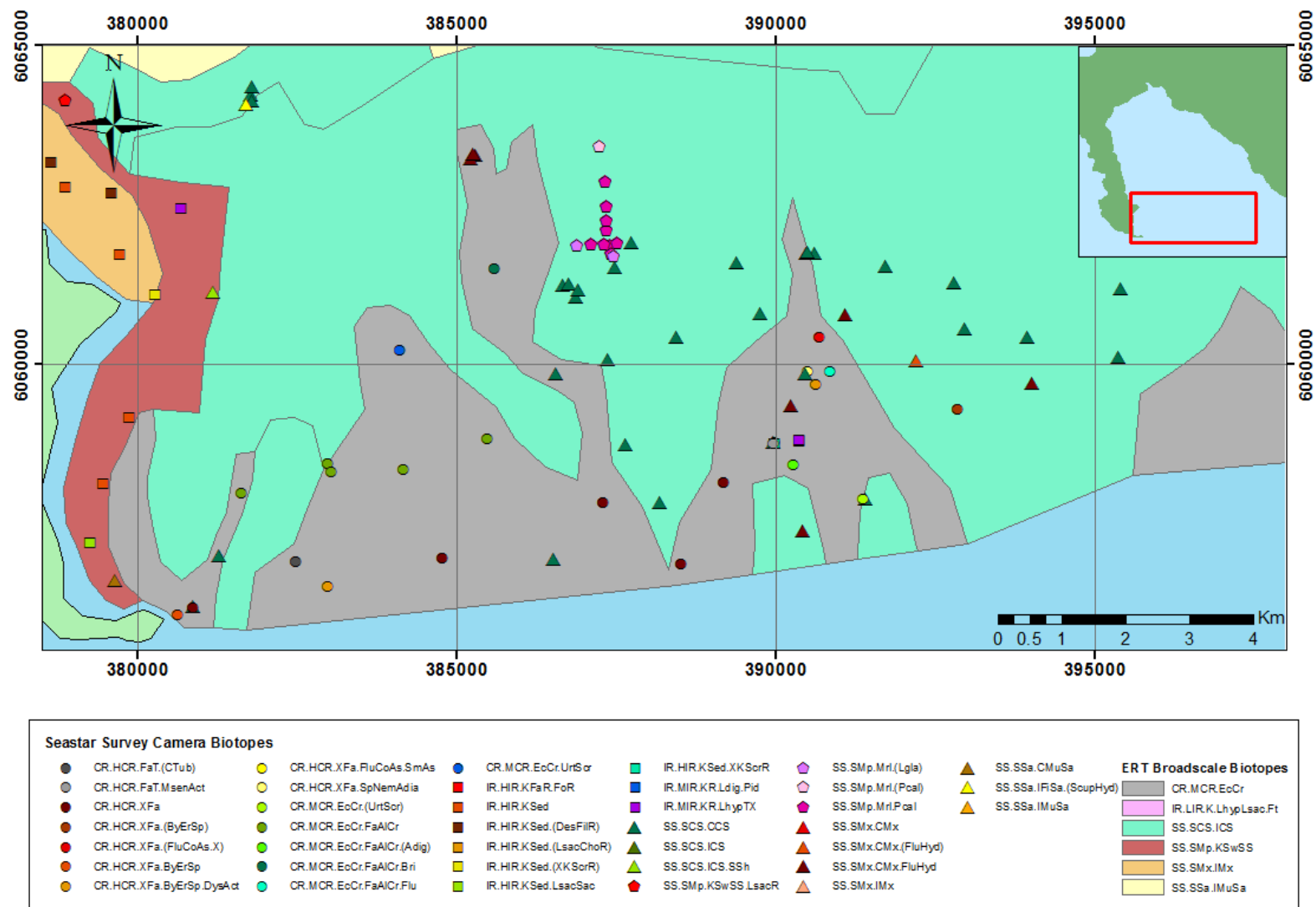
Figure 33. ERT Ltd. broadscale biotope map and Seastar Survey 2012 camera biotopes at the mouth of Luce Bay. © Crown copyright and database rights [2014] Ordnance Survey 100017908.
