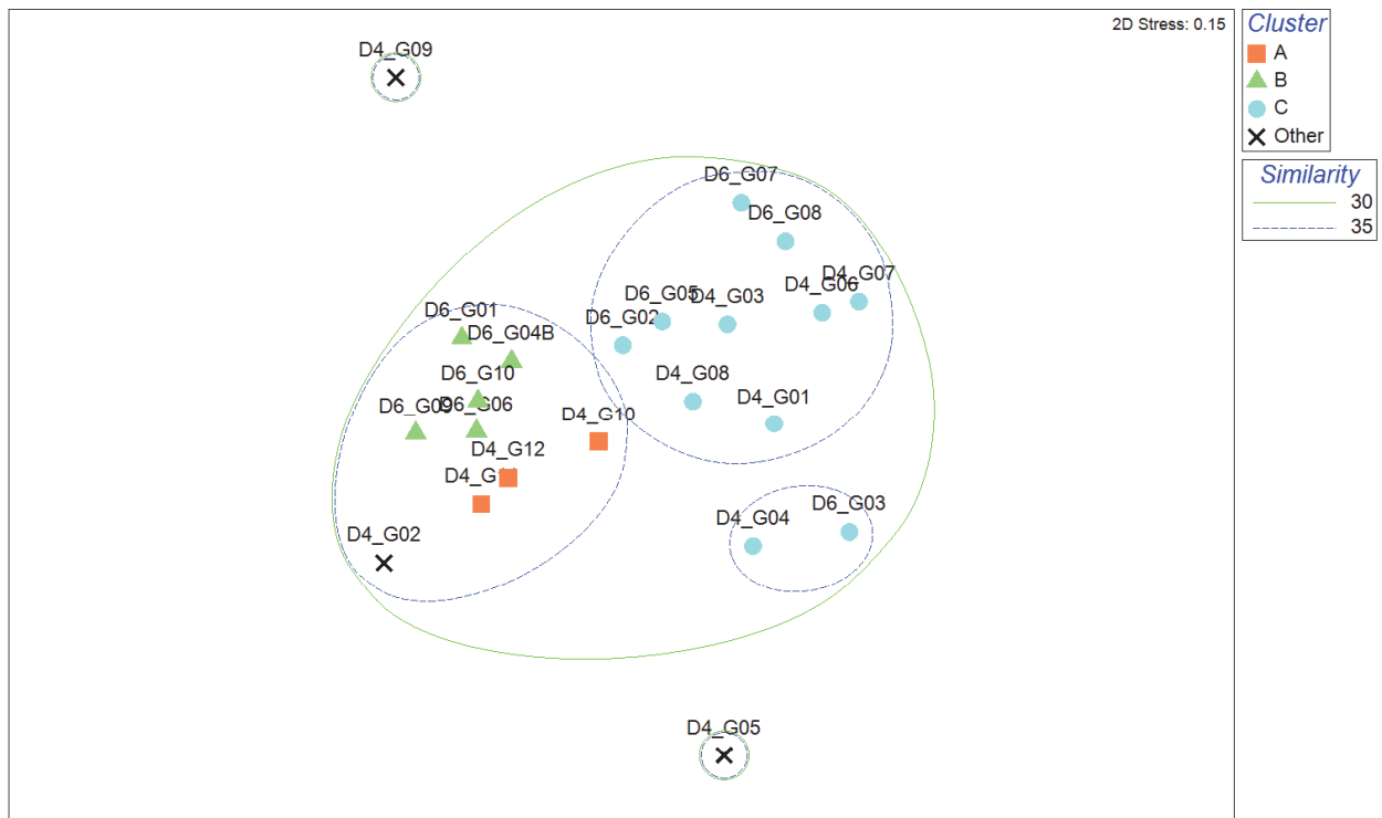
Figure 3.5: Ordination analysis of the macrobenthic invertebrate sample data from stations D4 and D6 collected from South Arran NC MPA in 2015.
